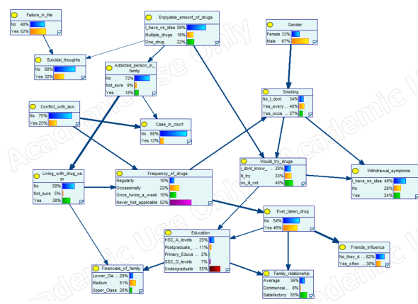
Fig. 2. Bayesian Network for Predicting “Frequency of Drugs” Visualized in GeNIe.
