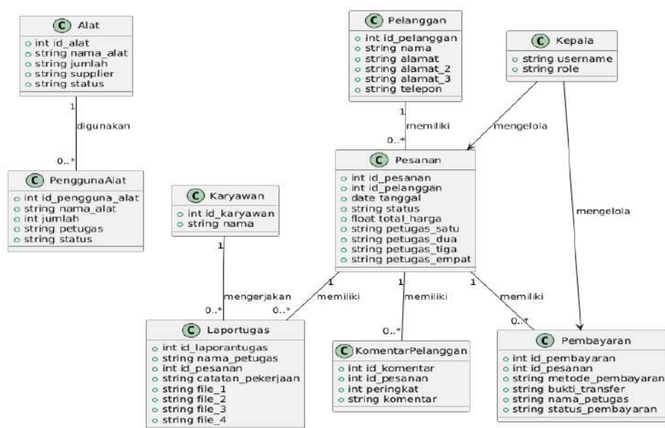
Gambar 3. 8 Class Diagram
