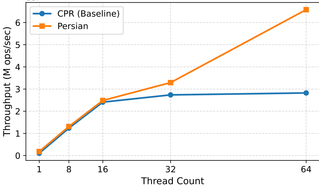
1e7 Throughput Comparison under R90/W10 Workload
