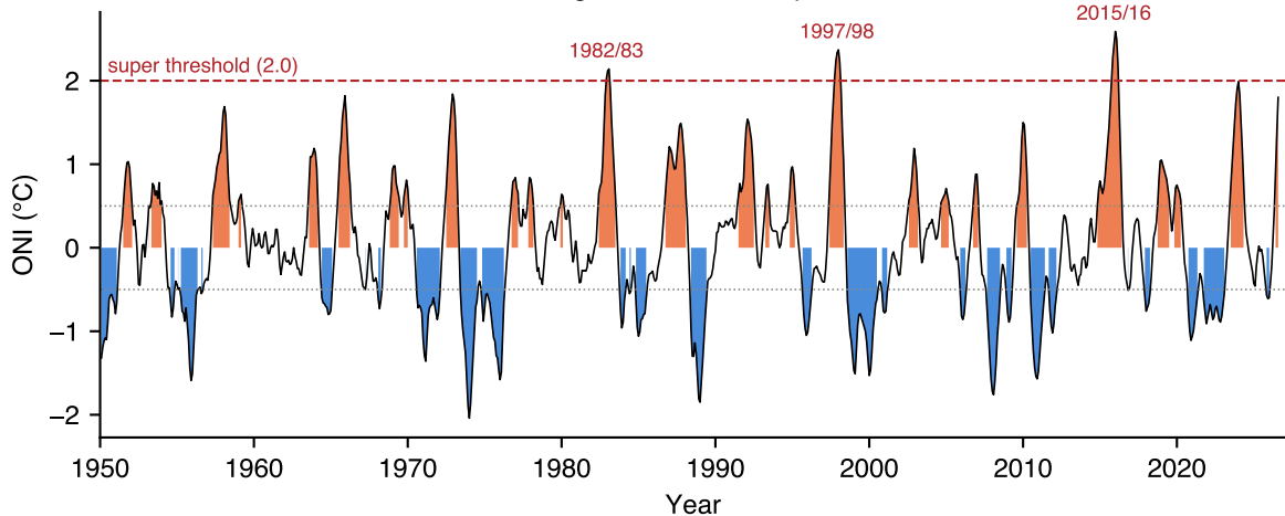
Oceanic Niño Index, 3-month running mean, 1950 to present
