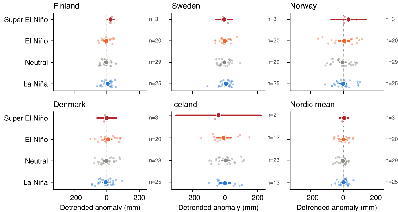
Precipitation sum (mm), DJF: group means with 95% CI
