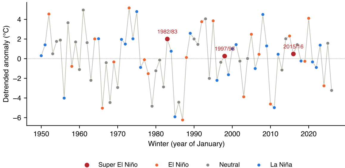
Finland: Mean temperature ( ^{\circ}\text{C} ), DJF
