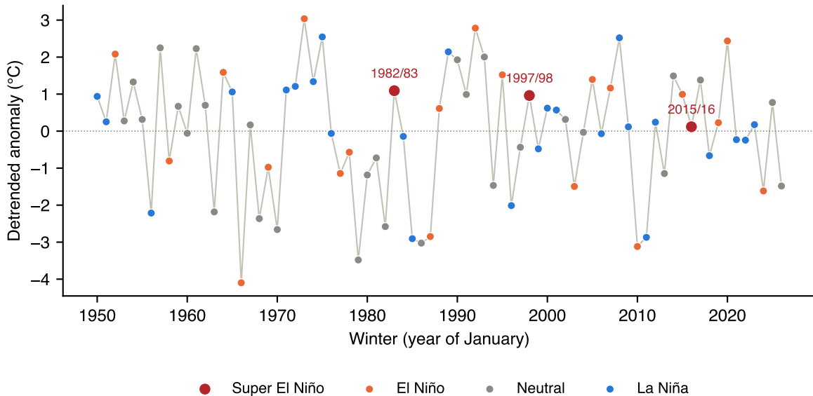
Nordic mean: Mean temperature ( ^{\circ}\text{C} ), DJF
