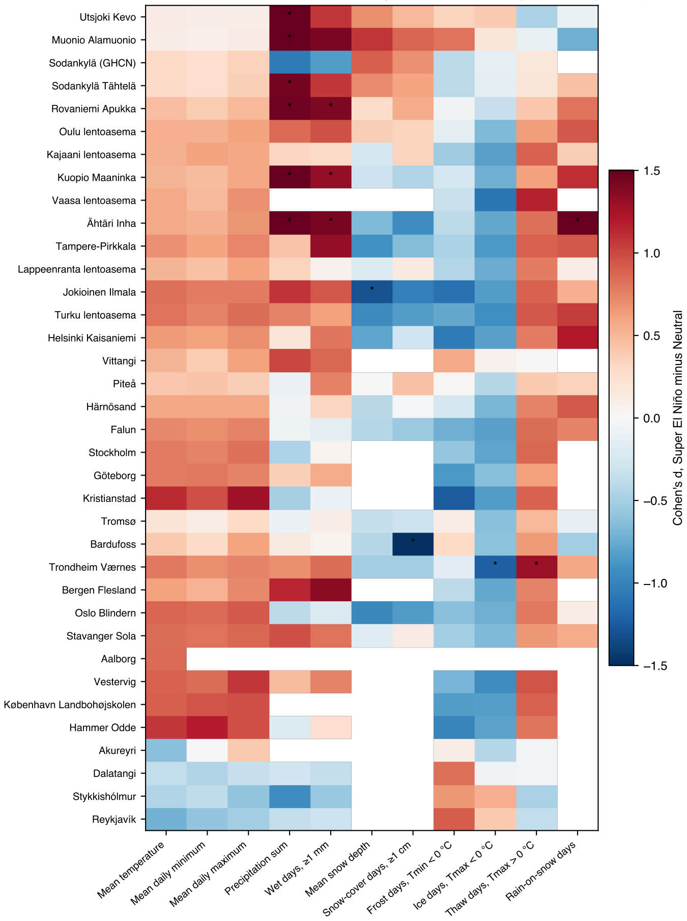
DJF, detrended anomalies: effect size by station and metric (* permutation p < 0.05)
