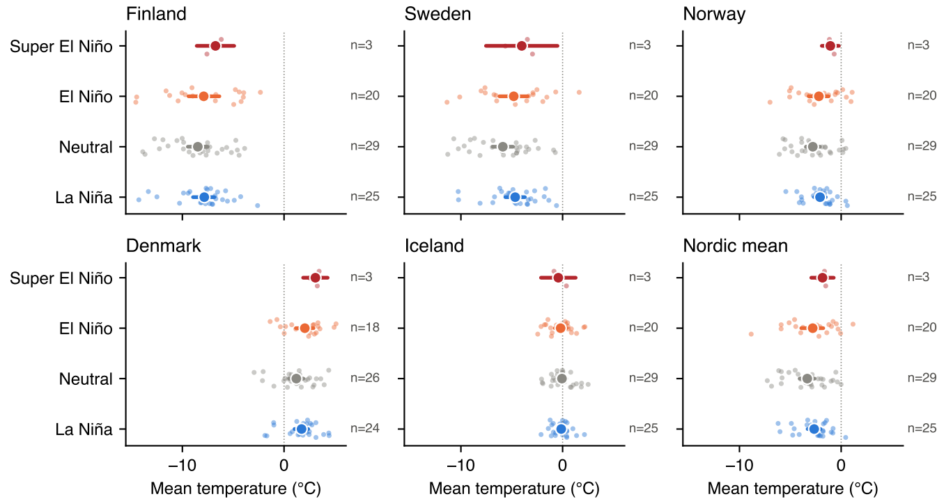
Mean temperature (°C), DJF: group means with 95% CI
