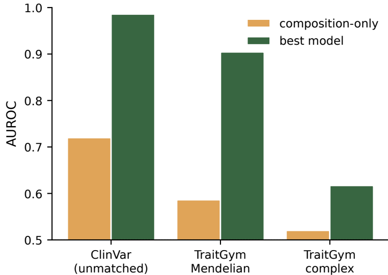
(b) Absolute AUROC: composition vs best model
