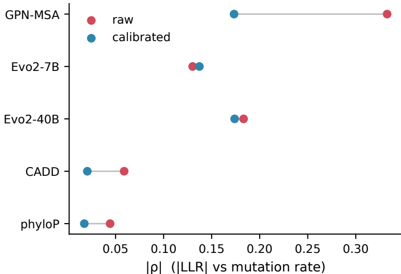
(a) ClinVar: mutation-rate coupling before→after calibration
