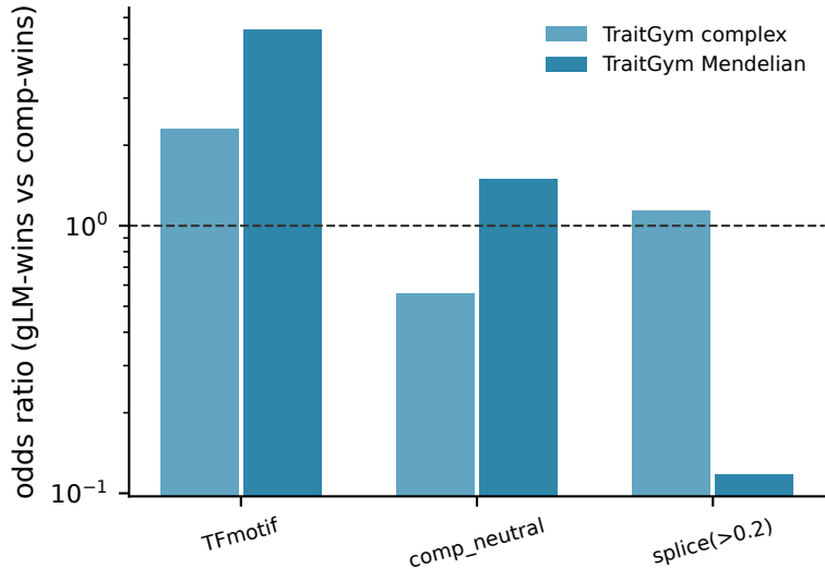
(b) Surviving signal: gLM-wins enriched for TF motifs
