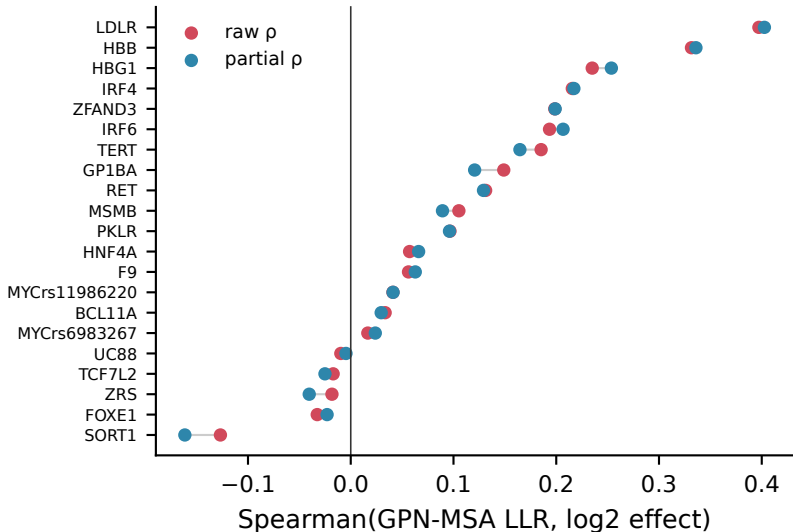
(a) Kircher within-element: partial \approx raw (no leakage)
