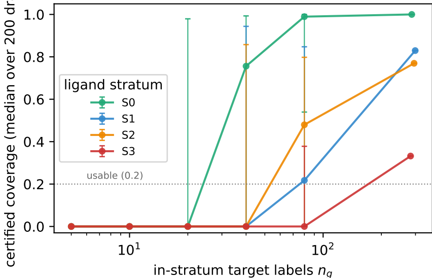
Label-cost curve (AF3, combined score): certified coverage bought per stratum by n_g labels
