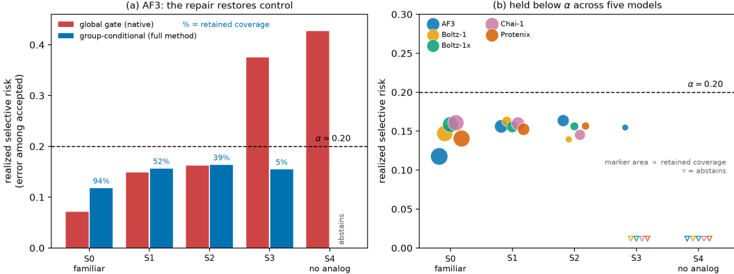
Figure 3: The repair. Group-conditional calibration holds realized selective risk at or below \alpha = 0.20 on the strata where the marginal gate over-shoots, folding to zero coverage on the no-analog tail rather than issuing a false certificate. Coverage labels are direct; the coverage cost grows with novelty.
