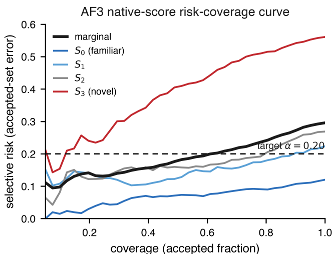
Figure 2: The break as an operating characteristic. AF3 native-score selective risk against coverage, marginal and per ligand-novelty stratum (point estimates). The familiar stratum S_0 stays far below \alpha at every coverage; the novel stratum S_3 sits above \alpha except at the lowest coverage, and S_4 (omitted for scale) is above it throughout. The certified frontier of Sec. 4 is stricter still, since it reads the Clopper-Pearson upper bound under a \geq 20 -accept rule rather than these point estimates.
