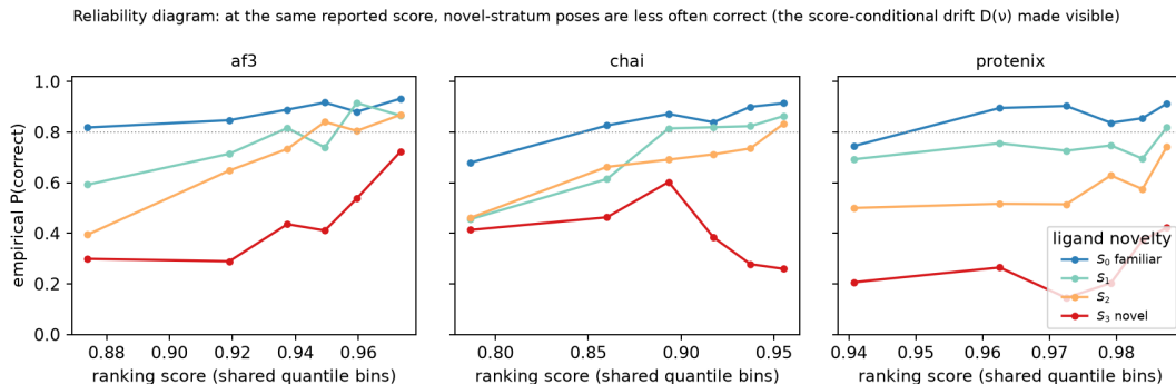
Figure 2: Reliability diagram. Empirical P(\text{correct}) against the frozen ranking score (shared quantile bins), one curve per ligand-novelty stratum. The curves stay monotone (the score discriminates within each stratum, so the gate is not anti-selective) but drop together on novel strata (the base rate collapses), the visible form of the score-conditional reliability drift D(v) .
