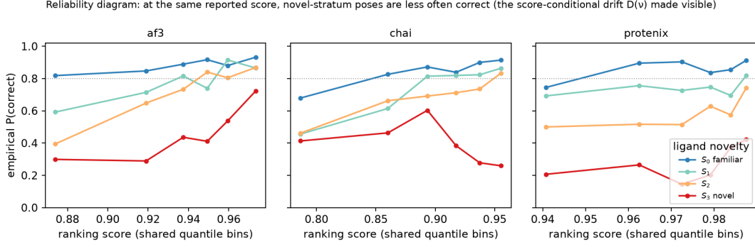
Figure S2: Reliability diagram. Empirical P(\text{correct}) against the frozen ranking score (shared quantile bins), one curve per ligand-novelty stratum. The curves stay monotone (the score discriminates within each stratum, so the gate is not anti-selective) but drop together on novel strata (the base rate collapses), the visible form of the score-conditional reliability drift D(v) .
