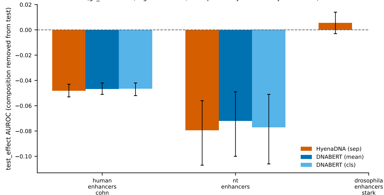
Cross-architecture: BOTH frozen FMs lose enhancer AUROC when composition is removed (gc_match arm, LightGBM head; drosophila = HyenaDNA-only flat control)
