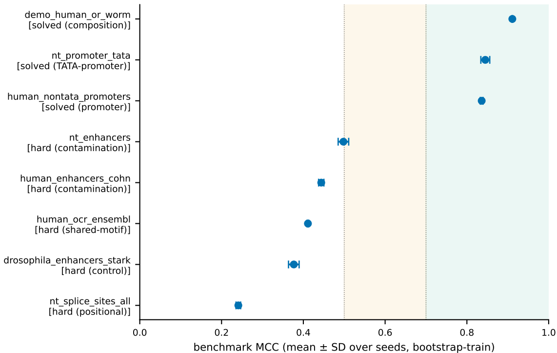
Multi-seed robustness: MCC is seed-invariant (max SD = 0.013)
