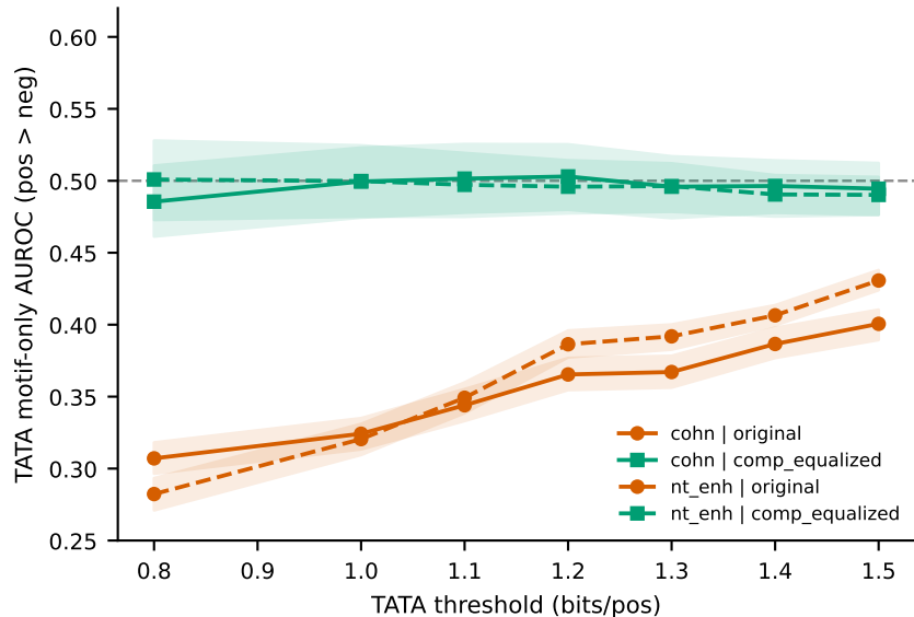
Threshold invariance original stays neg-skewed; comp-equalized flat on 0.5
