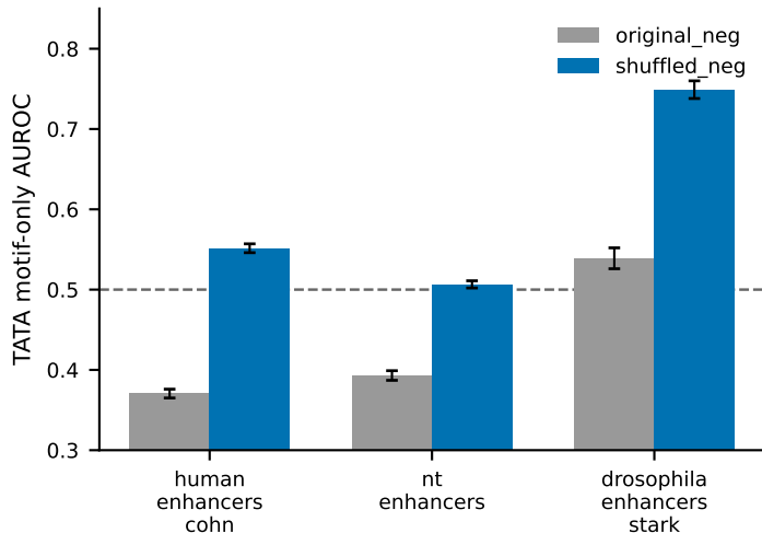
TATA artifact vs shuffled negatives
