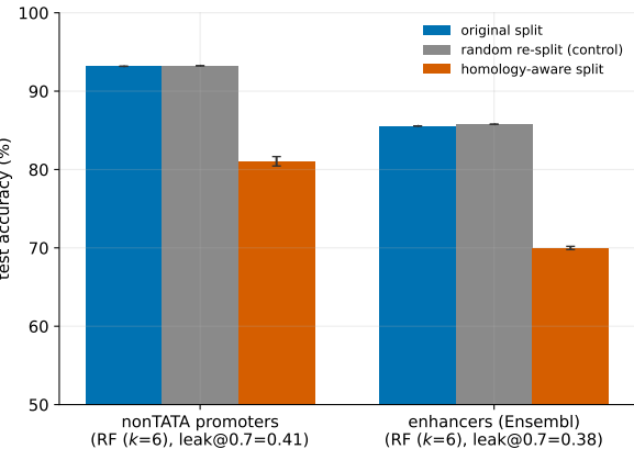
Negative control: only the homology-aware split removes the inflation
