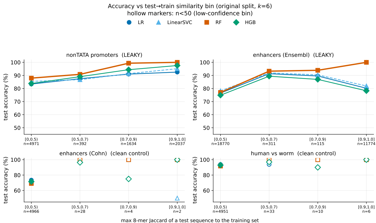
Figure S2: Accuracy as a function of the test-to-train similarity bin (as-shipped split, k=6 , the four-model comparison). On leaky datasets the near-default random forest is near-perfect on high-similarity (near-duplicate) test sequences and falls on dissimilar ones; clean controls have near-empty high-similarity bins. Hollow markers denote bins with n < 50 .
