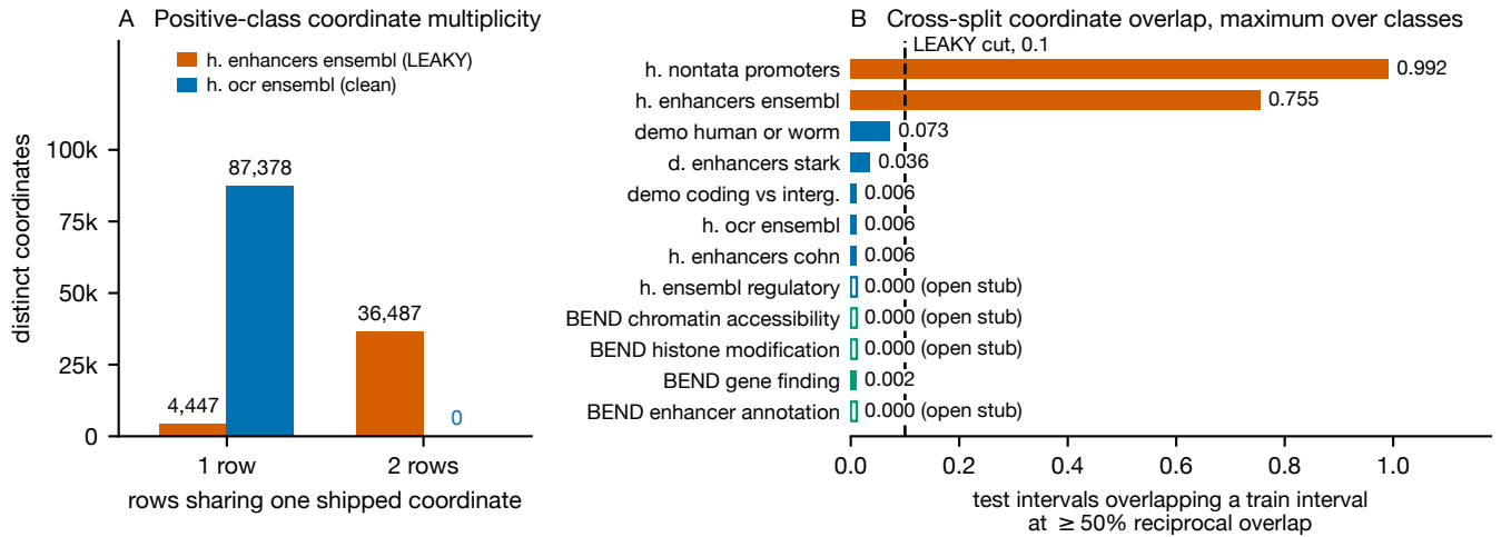
Figure 1 The construction defect in the shipped coordinates, measured before any model is trained. (A) Distinct positive-class coordinates by the number of rows sharing them, for the leaky human_enhancers_ensembl and the clean human_ocr_ensembl ; 36,487 of the former’s coordinates carry two rows each, 94.3% of its positive rows. (B) Fraction of test intervals overlapping any training interval at \geq 50\% reciprocal overlap, taken as the maximum over classes, for the eight Genomic Benchmarks datasets and the four BEND partitions (green); the dashed rule at 0.1 is the LEAKY cut used throughout, carried over unchanged from sequence space, so the screen adds no fitted parameter. A measured 0.000 is drawn as an open hairline stub and labelled as such, so that it is distinguishable both from a small non-zero bar and from a missing one; four partitions read exactly zero. Overlap is strand-agnostic. demo_coding_vs_intergenomic_seqs is the one miss: it is borderline in sequence space under containment, but one of its classes is keyed by transcript accession rather than by interval, so its 0.006 is structurally zero rather than measured.
