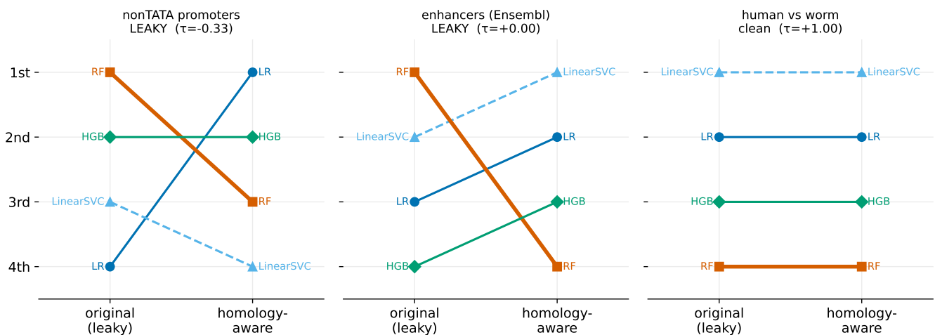
Figure 2 Model rankings on the original (leaky) split versus the homology-aware split ( k=6 , accuracy). The random forest is dethroned on the leaky datasets (left, middle) but rankings are stable on a clean control (right). Per-panel \tau is the rank correlation for that dataset; on enhancers (Ensembl) the random forest's move to last flips only its own pairs, giving \tau \approx 0 despite the dramatic demotion—illustrating why \tau is too coarse to serve as a primary statistic with only four models (§4.3).
