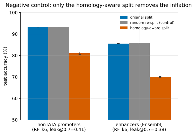
Figure 1 Original split versus random re-split (negative control) versus homology-aware re-split, best model per dataset. Only the homology-aware split lowers accuracy, and only on leaky datasets. The y -axis is truncated at 50% (not 0%) to make the homology-aware accuracy drop visible; bars span best-model accuracies of roughly 70–93%.
