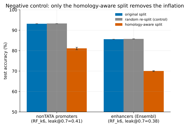
Figure 2 Original split versus random re-split (negative control) versus homology-aware re-split, best model per dataset. Only the homology-aware split lowers accuracy, and only on leaky datasets.
