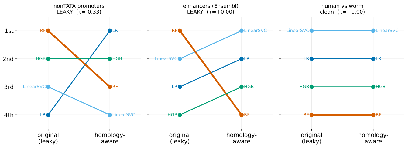
Figure 3 Model rankings on the original (leaky) split versus the homology-aware split ( k=6 , accuracy). The random forest is dethroned on the leaky datasets (left, middle) but rankings are stable on a clean control (right).
