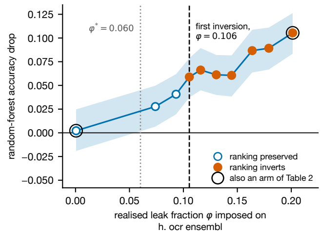
Figure 2 Ten doses of the same construction defect, imposed on the clean human_ocr_ensembl . Random-forest accuracy drop under near-duplicate-aware correction against the realised test-set leak fraction \varphi at Jaccard 0.9; the shaded band is the two-arm cluster-bootstrap 95% CI over whole within-test near-duplicate components, and each dose is a single fit at one split seed. Filled points are doses at which the four-model ranking inverts, open points doses at which it does not. Circled points are the two arms of Table 2 re-reported rather than fresh trials, so the sweep supplies eight additional doses. The dashed rule marks the first inversion, the dotted rule the diagnostic threshold \varphi^* computed at that dose.
