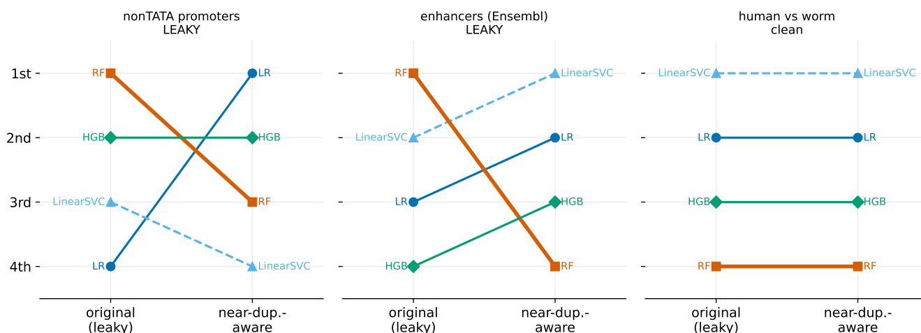
Figure 3 Four-model rankings on the original (leaky) split versus the near-duplicate-aware split ( k=6 , accuracy). The random forest is dethroned on human_enhancers_ensembl (middle) and, under accuracy only, on human_nontata_promoters (left), while rankings are stable on the clean control demo_human_or_worm (right, 20k subsample). Kendall \tau is deliberately not annotated: at four models it is too coarse to carry (§3.5), and it orders these panels opposite to the conclusions they support.
