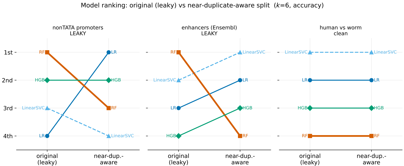
Figure 3 Four-model rankings on the original (leaky) split versus the near-duplicate-aware split ( k=6 , accuracy). The random forest is dethroned on human_enhancers_ensembl (middle) and, under accuracy only, on human_nontata_promoters (left), while rankings are stable on the clean control demo_human_or_worm (right, 20k subsample). Kendall \tau is deliberately not annotated: at four models it is too coarse to carry (§3.6), and it orders these panels opposite to the conclusions they support.
