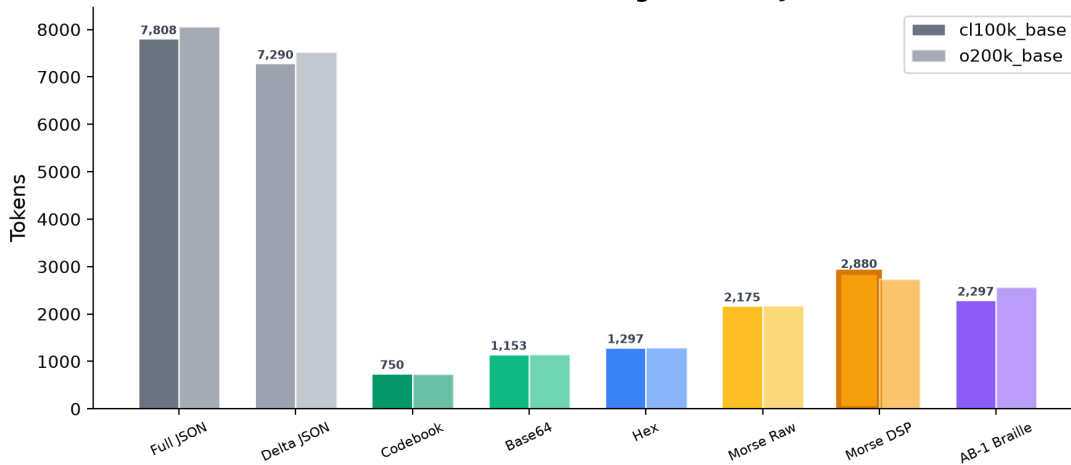
Figure 4: Real agent trace comparison (235 self-harness traces, 8-byte states, 82.5% change rate). Morse DSP achieves 60.8% savings vs delta JSON.
