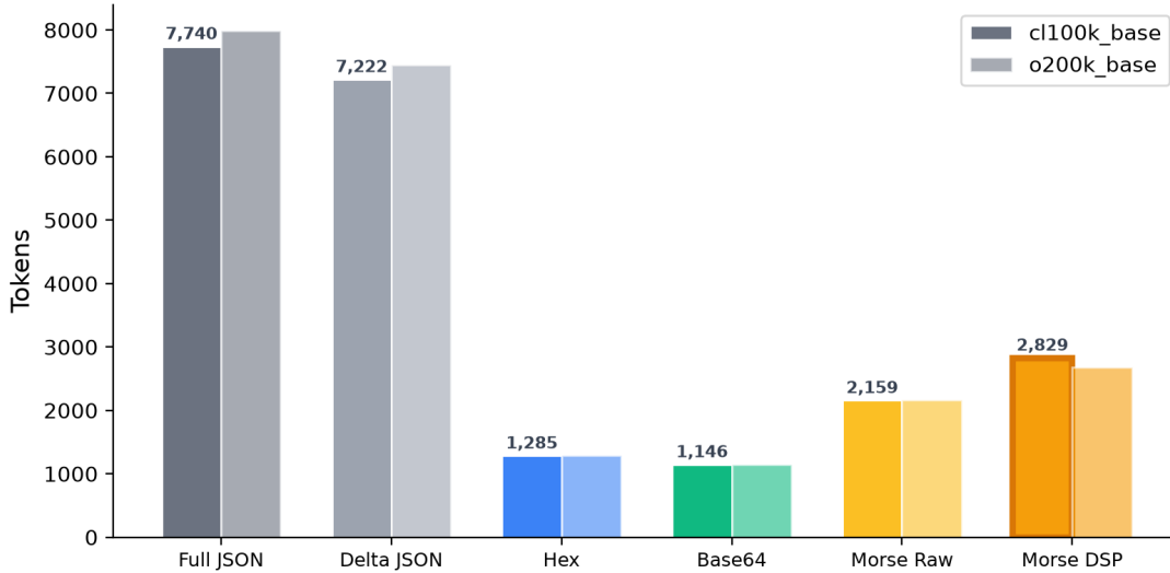
Fig. 4: Real Self-Harness Traces — 235 traces, 8-byte states Morse DSP: 60.8% savings vs Delta JSON
