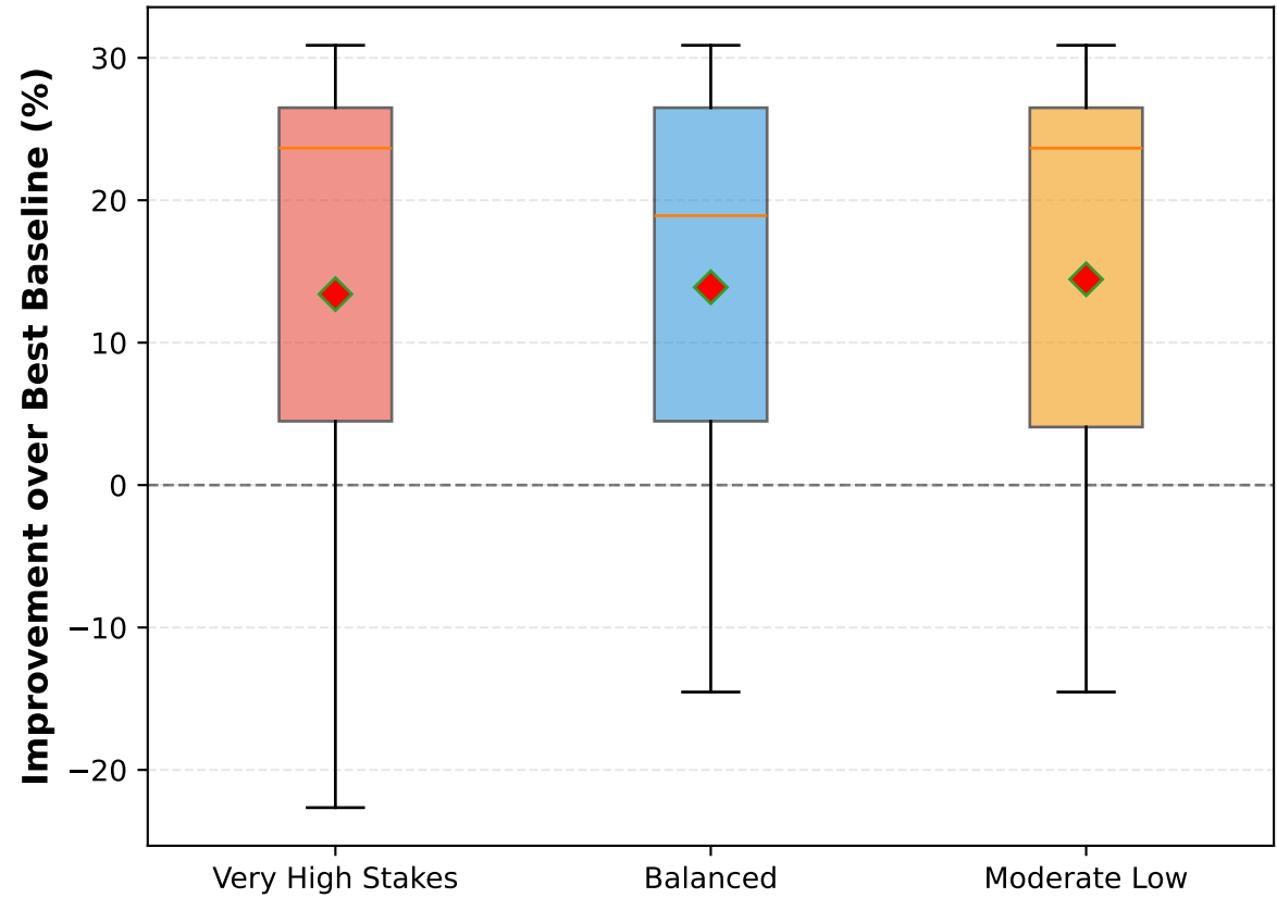
Improvement % Distribution by Regime
