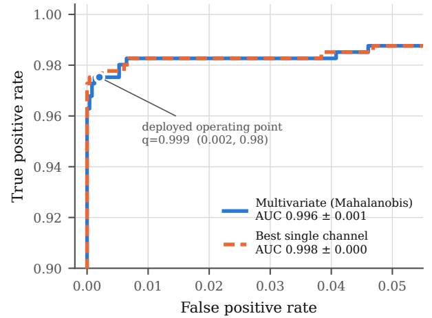
Fig. 4. Telemetry-plane ROC on the attacked runs, zoomed to \text{FPR} \leq 0.055 ; over the full range the two curves are indistinguishable. AUC is the mean \pm s.d. over 20 trials. The per-channel detector is marginally better than the multivariate one.
