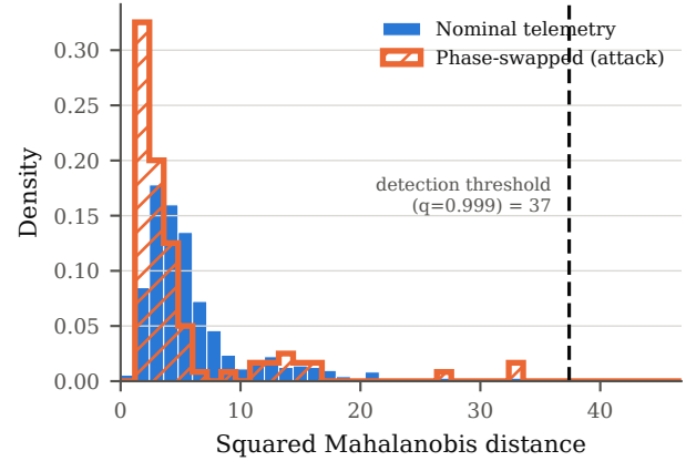
Fig. 3. Score distributions under the phase-swap probe. Replayed housekeeping frames from half an orbit earlier sit inside, and in fact below, the nominal distribution, because orbit phase is marginalised away by a baseline fitted over a whole orbit. Texture is redundant with colour for grayscale printing.
