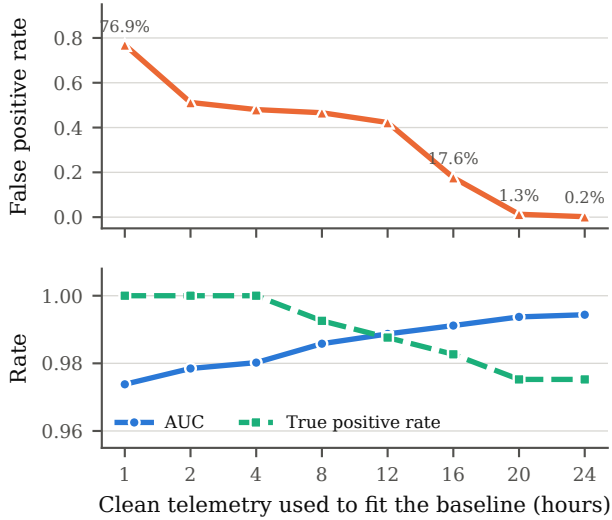
Fig. 4. Baseline-size sensitivity. Upper panel: telemetry false-positive rate at the deployed operating point. Lower panel: area under the curve and true-positive rate. The false-positive rate collapses only when the training window covers a full diurnal cycle; discrimination barely changes.
