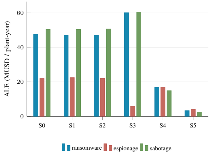
Fig. 6. Annualised loss expectancy per control scenario and actor profile. Scenario S_3 lowers espionage risk sharply while increasing ransomware risk: hardening the cheap data-theft routes displaces a rational actor onto the availability objective.
