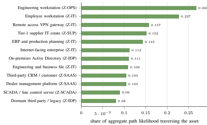
Fig. 5. Likelihood-weighted choke points of the reference architecture.
