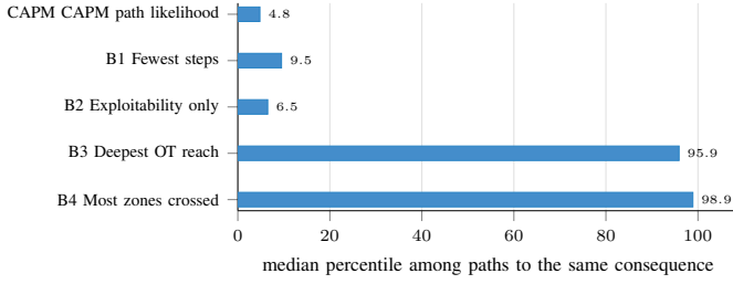
Fig. 10. Median percentile of the corpus incidents under each prioritisation (lower is better). The segmentation- and depth-centric heuristics rank the routes that actually occurred near the bottom of their lists.
