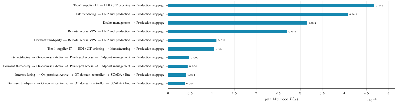
Fig. 3. Ten most likely attack paths to production stoppage in the baseline configuration S_0 . The highest-likelihood routes terminate in business and logistics systems, not in controllers.
