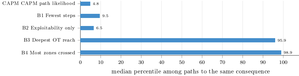
Figure 10: Median percentile of the corpus incidents under each prioritisation (lower is better). The segmentation- and depth-centric heuristics rank the routes that actually occurred near the bottom of their lists.
