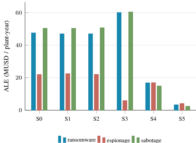
Fig. 6. Annualised loss expectancy per control scenario and actor profile. Scenario S_3 lowers espionage risk sharply while increasing ransomware risk: hardening the cheap data-theft routes displaces a rational actor onto the availability objective.
