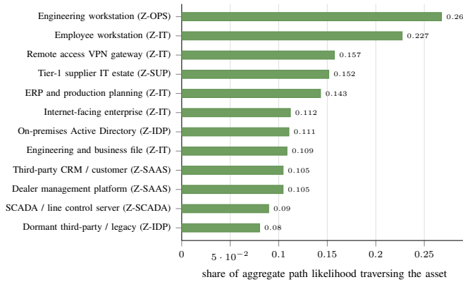
Fig. 6. Likelihood-weighted choke points of the reference architecture.
