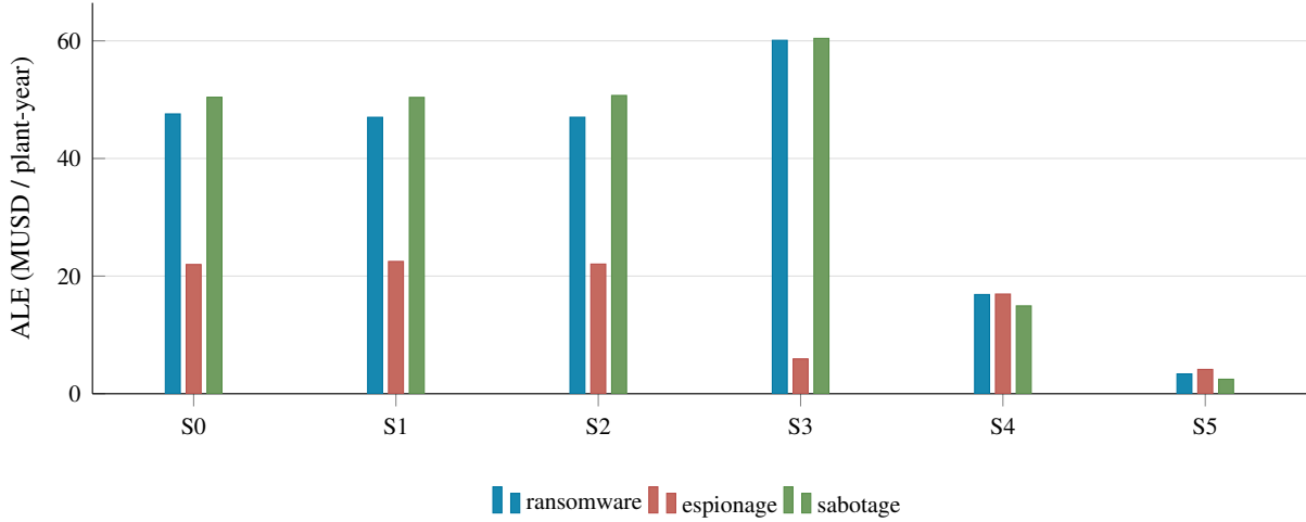
Figure 8: Annualised loss expectancy per control scenario and actor profile. Scenario S_3 lowers espionage risk sharply while increasing ransomware risk: hardening the cheap data-theft routes displaces a rational actor onto the availability objective.
