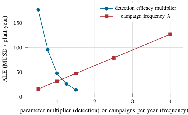
Fig. 9. One-at-a-time sensitivity of the annualised loss expectancy. Halving detection efficacy multiplies the baseline ALE by 3.7; the response to campaign frequency is linear by construction.
