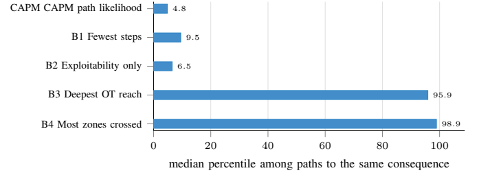
Fig. 10. Median percentile of the corpus incidents under each prioritisation (lower is better). The segmentation- and depth-centric heuristics rank the routes that actually occurred near the bottom of their lists.
