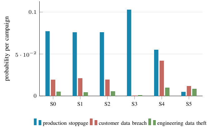
Fig. 7. Consequence mix per campaign under each control scenario, big-game ransomware profile. S_3 removes the cheap data-theft outcomes and the production-stoppage probability rises: the displacement effect of section VI.D made visible.
