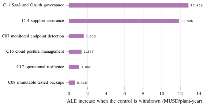
Fig. 9. Necessity of each control inside the full programme S_5 : the annualised loss that returns when that control alone is withdrawn.
