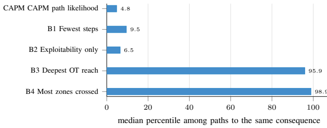
Fig. 12. Median percentile of the corpus incidents under each prioritisation (lower is better). The segmentation- and depth-centric heuristics rank the routes that actually occurred near the bottom of their lists.
