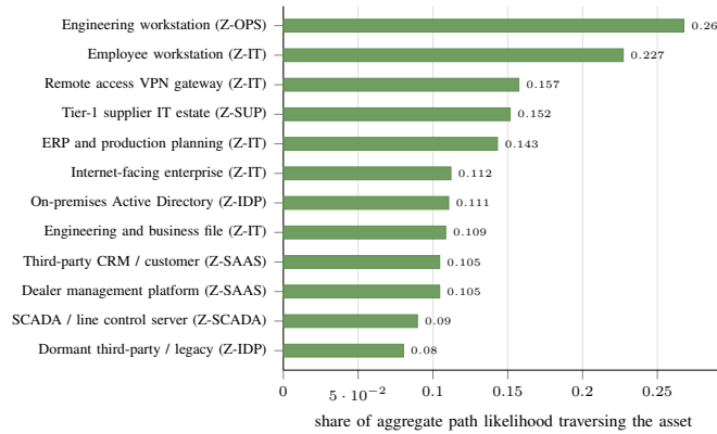
Fig. 6. Likelihood-weighted choke points of the reference architecture.
