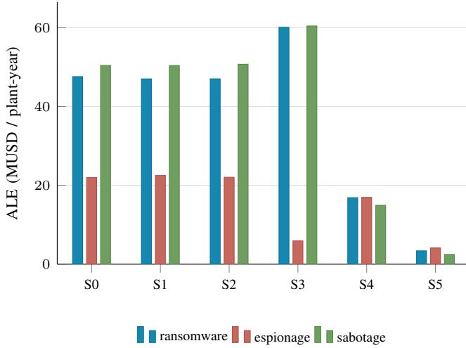
Fig. 8. Annualised loss expectancy per control scenario and actor profile. Scenario S_3 lowers espionage risk sharply while increasing ransomware risk: hardening the cheap data-theft routes displaces a rational actor onto the availability objective.
