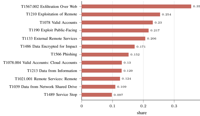
Fig. 5. MITRE ATT&CK techniques ranked by the share of aggregate path likelihood that traverses them (Enterprise and ICS matrices combined).
