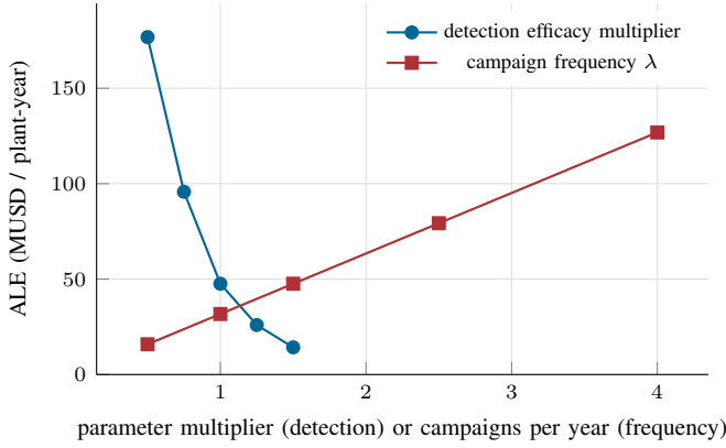
Fig. 11. One-at-a-time sensitivity of the annualised loss expectancy. Halving detection efficacy multiplies the baseline ALE by 3.7; the response to campaign frequency is linear by construction.
