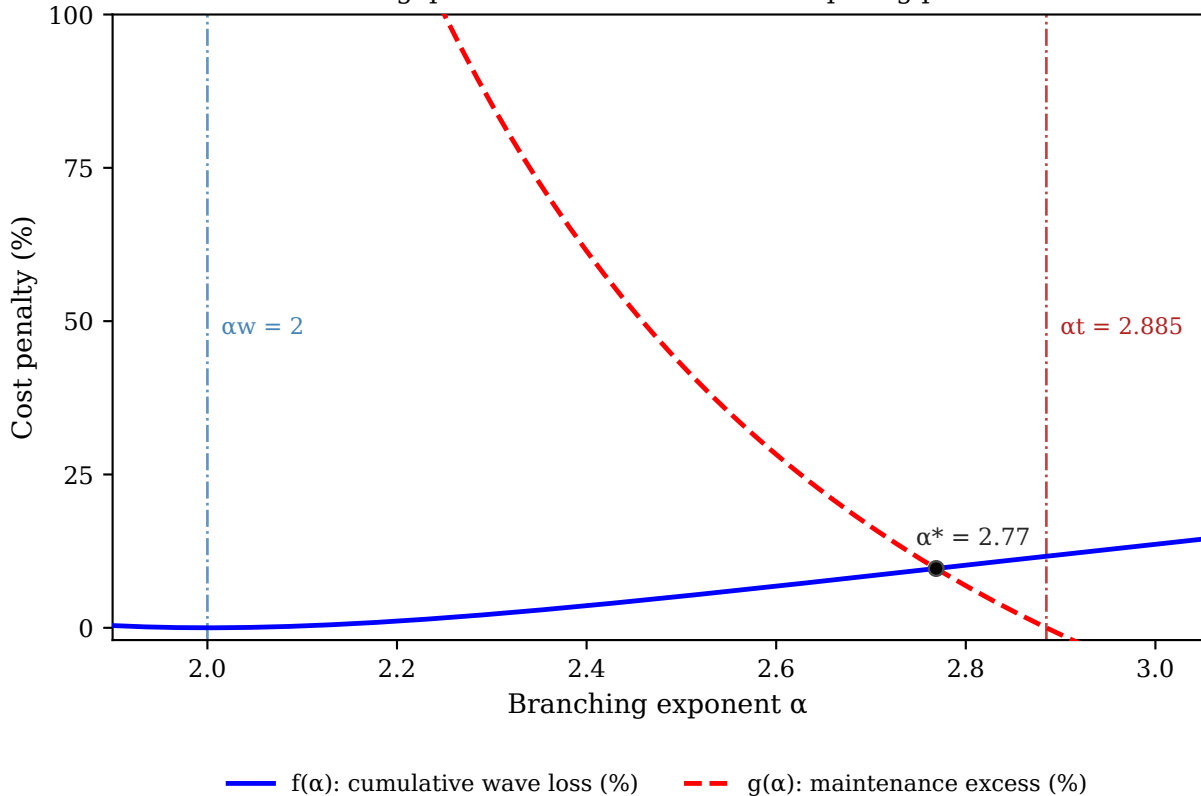
Minimax gap: wave vs. maintenance competing penalties
