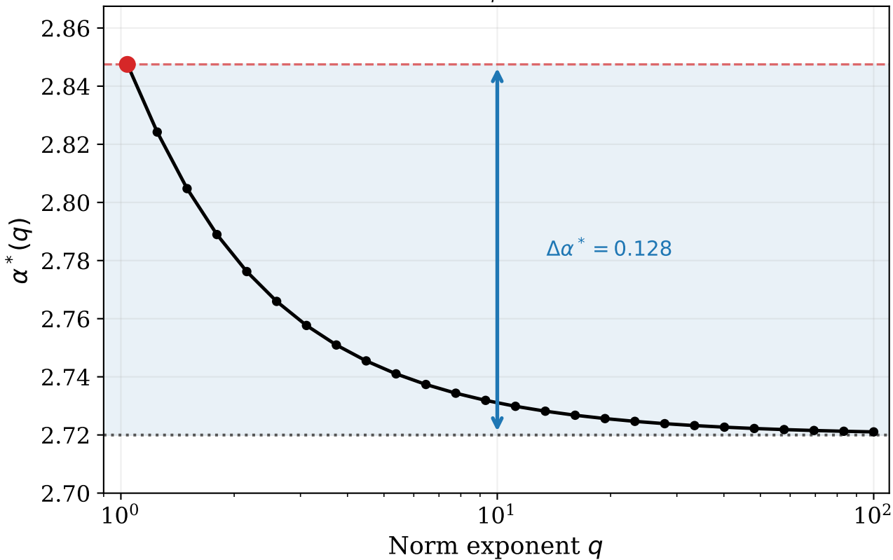
Robustness under L_q scalarization ( q \geq 1 )
