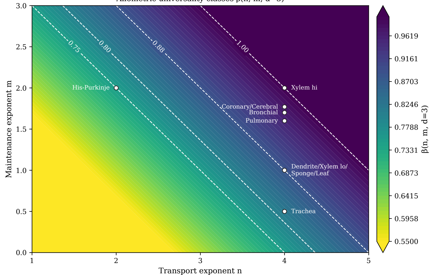
Allometric universality classes \beta(n, m, d=3)
