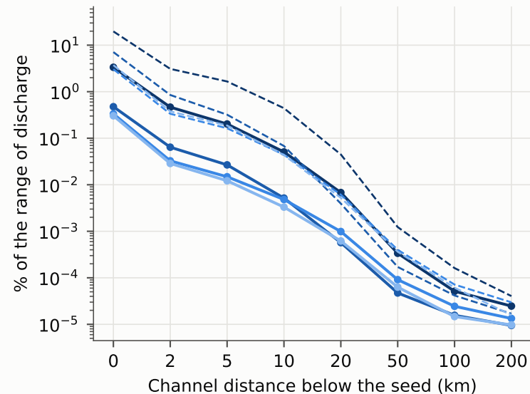
Alternating part difference, \Delta t = 1 h
