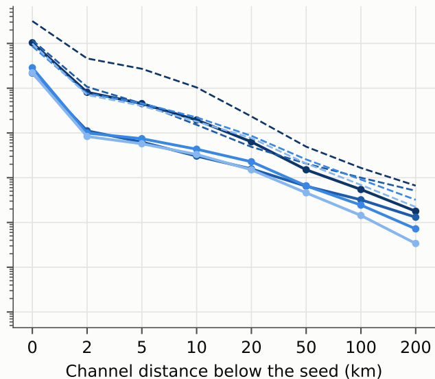
Largest difference, \Delta t = 1 h
