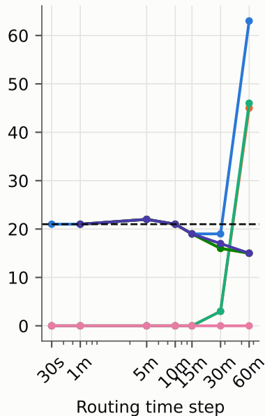
Rivers with negative discharge, burst
