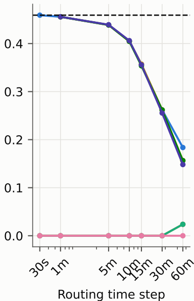
Rivers dipping > 1% of rise, burst (%)
