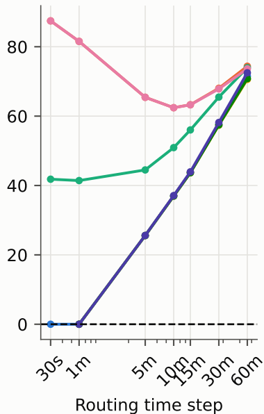
Rivers with alternating error > 1% of rise, square (%)
