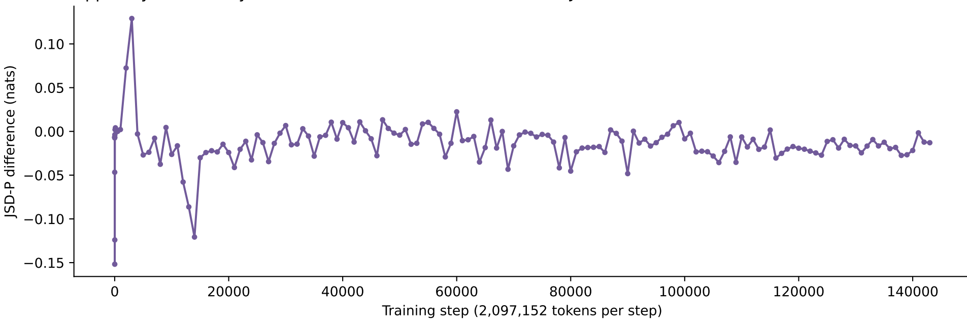
Apple-style discovery subset: female – male correct-answer JSD-P
