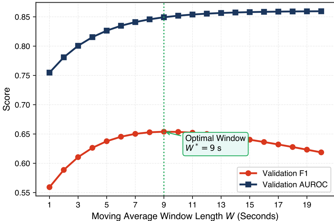
(A) Temporal Probability Smoothing Sweep
