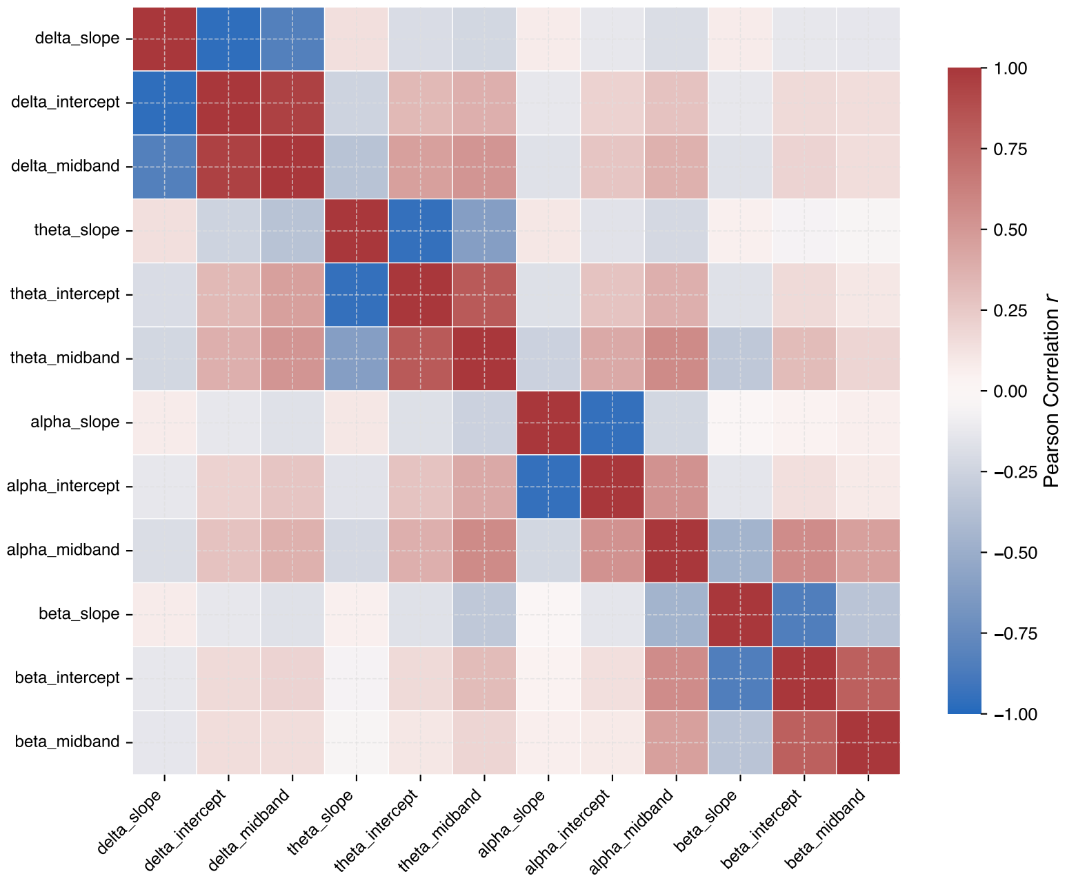
Study Feature Correlation Structure (Inter-Band Dynamics)
