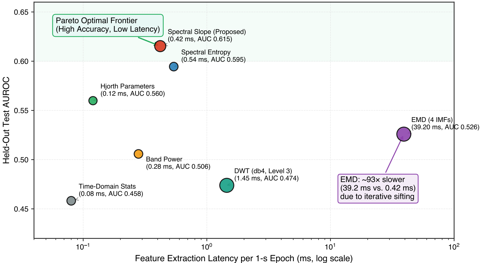
Computational Efficiency vs. Diagnostic Accuracy (Linear Classifier)
