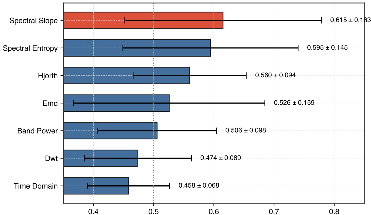
Test AUROC: Spectral Slope vs. Baselines
